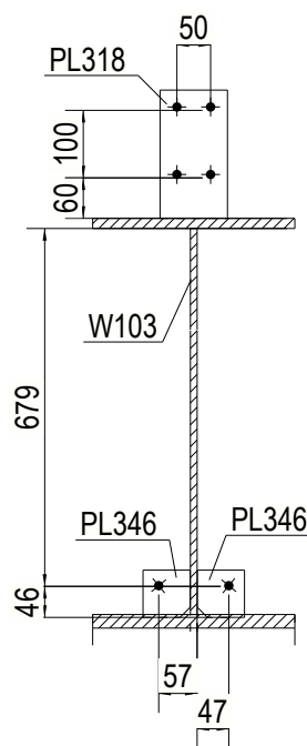
SEC A 1:12
