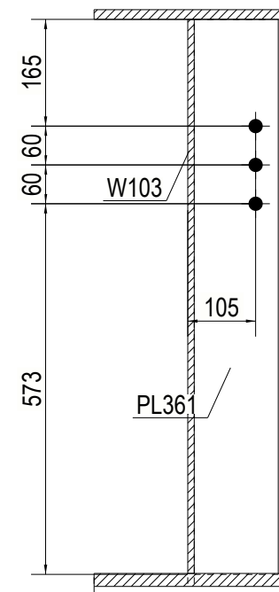
SEC B 1:10
